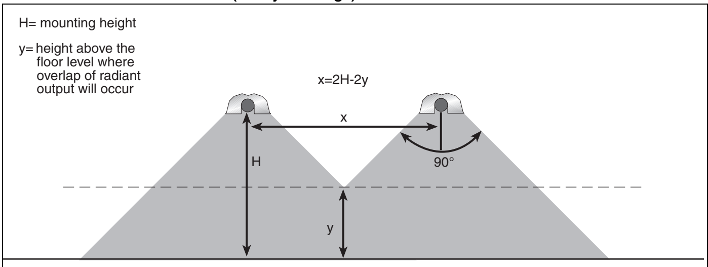
FIGURE 13: Radiant Distribution (Heavy Coverage)
